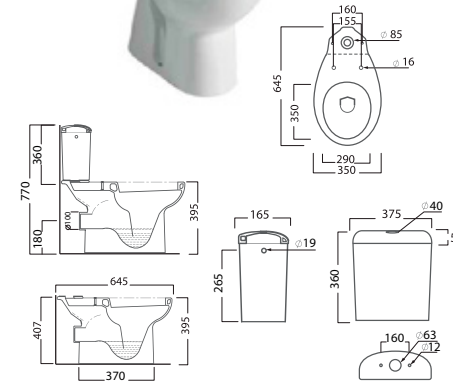
CLOSE COUPLED WC OLYMPIA
